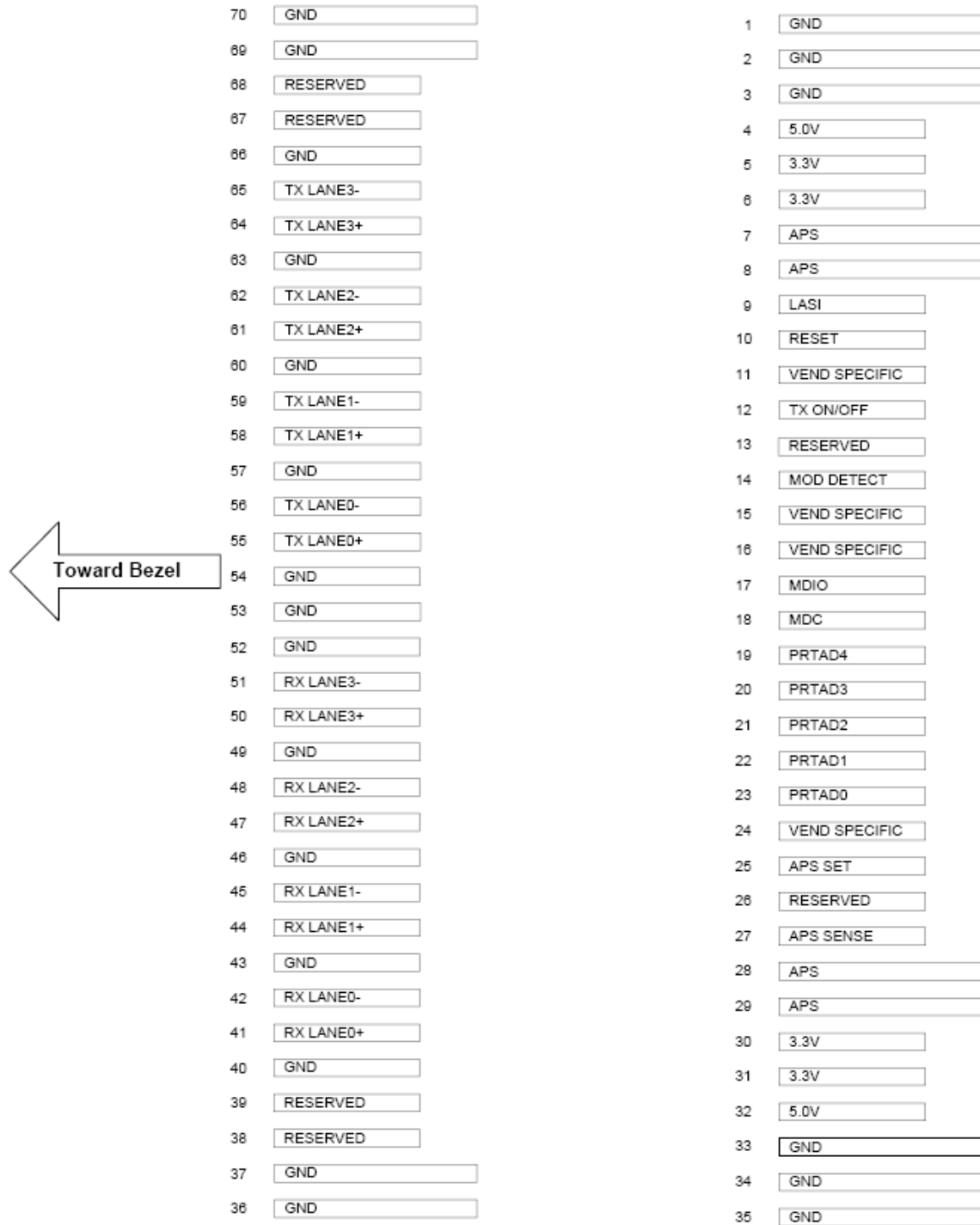
Figure2.Electrical Pin-out Details
